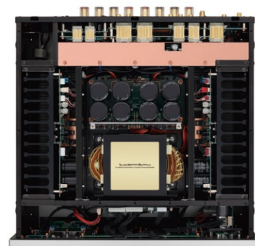
Internal configuration
